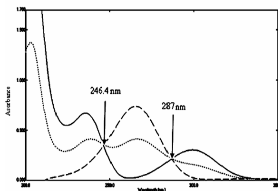
Fig. 4: Zero order absorption spectrum of 12 \mu\text{g mL}^{-1} Salicylamide (—), and 12 \mu\text{g mL}^{-1} Ascorbic acid (---) and mixture (salicylamide + Ascorbic acid 6 \mu\text{g mL}^{-1} of each) using double distilled water as a solvent.
