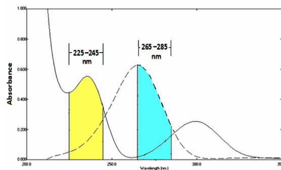
Fig. 3: Zero order absorption spectra of 10 \mu\text{g mL}^{-1} of Salicylamide (—) and 10 \mu\text{g mL}^{-1} of Ascorbic acid (----) showing wavelength ranges for AUC method using double distilled water as a blank
