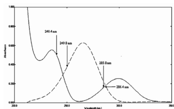
Fig. 2: Zero order absorption spectrum of 10 \mu\text{g mL}^{-1} of each of Salicylamide (—) and Ascorbic acid (----) using double distilled water as a solvent showing the selected wavelengths for dual wavelength method.
